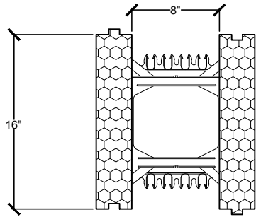
SECTION VIEW
