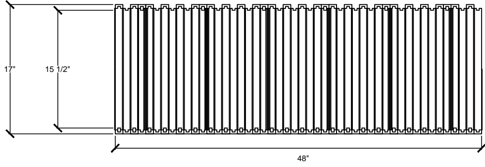
ELEVATION VIEW
