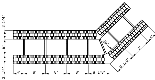
REVERSIBLE 45° CORNER BLOCK LEFT ORIENTED
