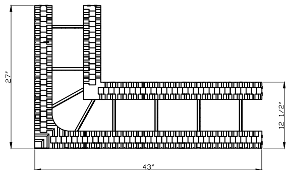
REVERSIBLE 90° CORNER BLOCK RIGHT ORIENTED
