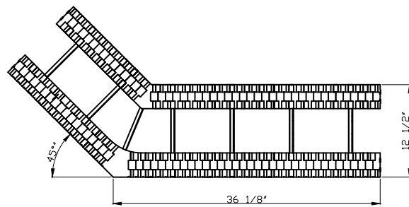
REVERSIBLE 45° CORNER BLOCK RIGHT ORIENTED
