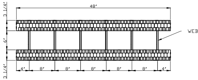
PLAN OF STRAIGHT BLOCK
