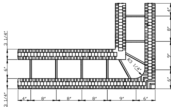
REVERSIBLE 90° CORNER BLOCK LEFT ORIENTED
