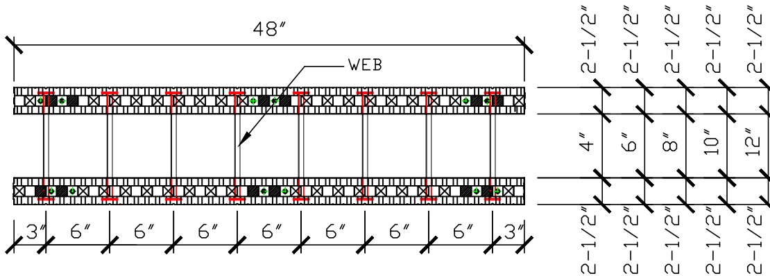
PLAN VIEW OF STRAIGHT BLOCK
