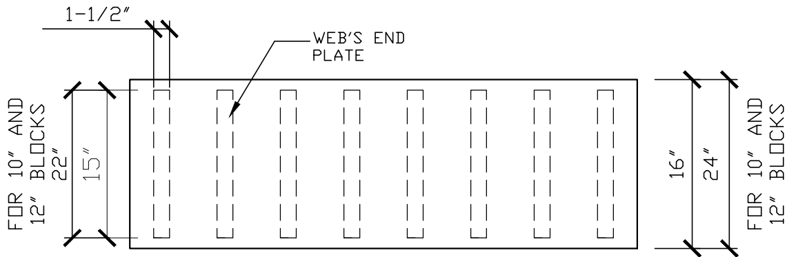
STRAIGHT BLOCK ELEVATION VIEW
