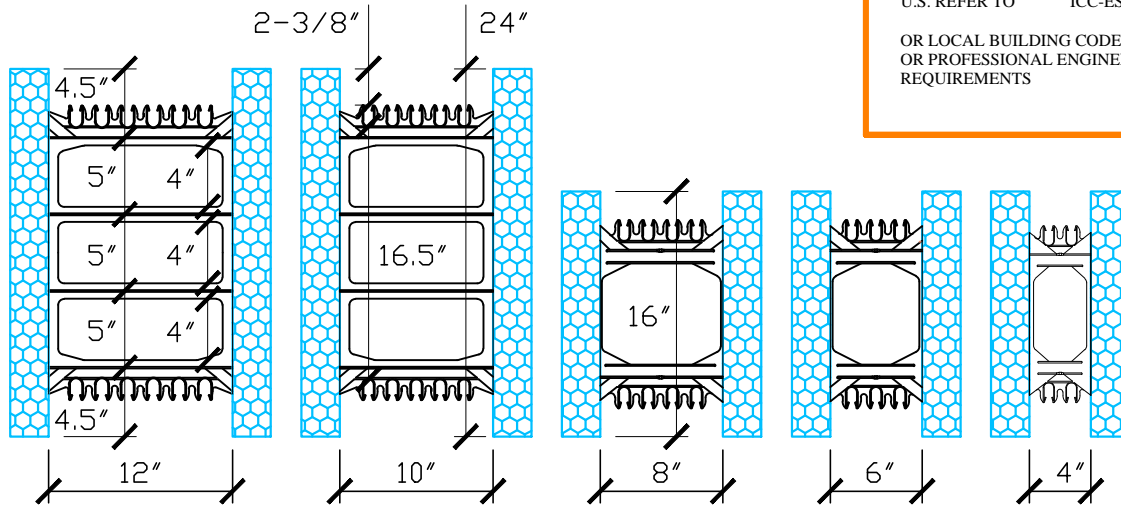
SECTION VIEW OF STRAIGHT BLOCKS
