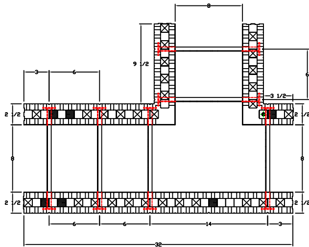
PLAN OF 8" T-BLOCK WITH SHORT LEG
