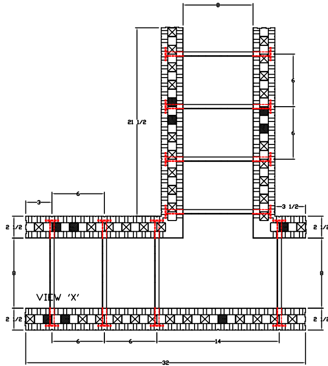
PLAN OF 8" T-BLOCK WITH LONG LEG
