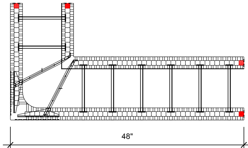
REVERSIBLE 90° LONG CORNER BLOCK RIGHT ORIENTED
