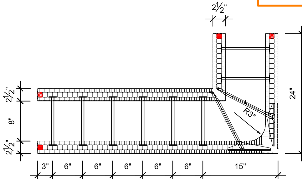
REVERSIBLE 90° LONG CORNER BLOCK LEFT ORIENTED
