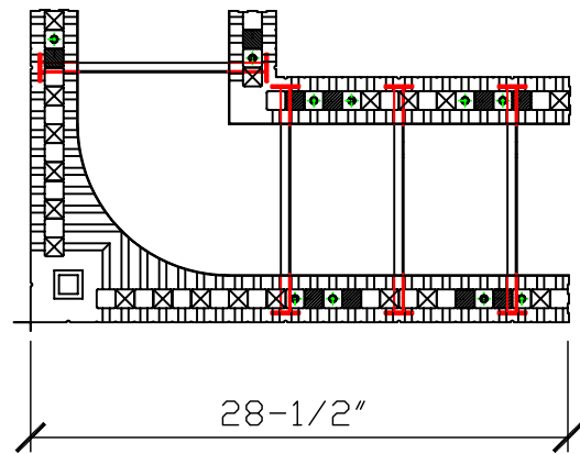
REVERSIBLE 90° CORNER BLOCK RIGHT ORIENTED
