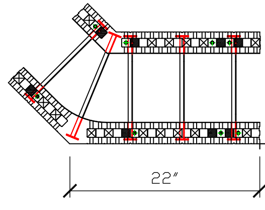
REVERSIBLE 45° CORNER BLOCK RIGHT ORIENTED
