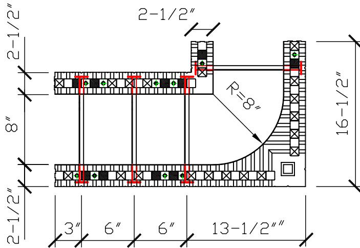
REVERSIBLE 90° CORNER BLOCK LEFT ORIENTED
