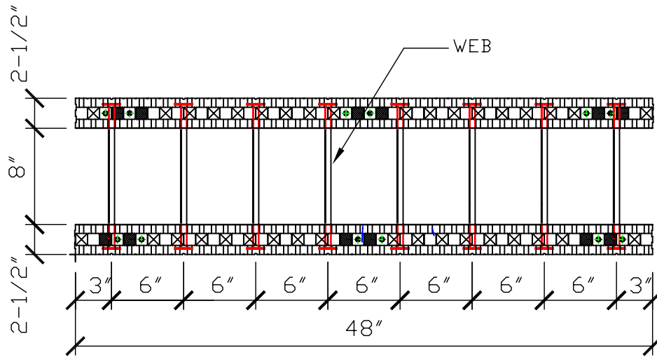
PLAN OF STRAIGHT BLOCK
