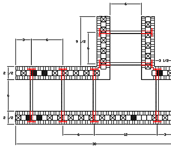
PLAN OF 6" T-BLOCK WITH SHORT LEG
