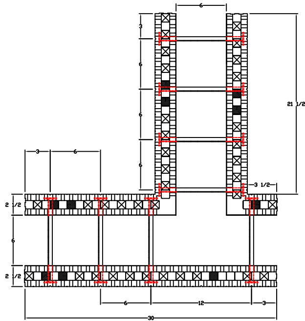
PLAN OF 6" T-BLOCK WITH LONG LEG
