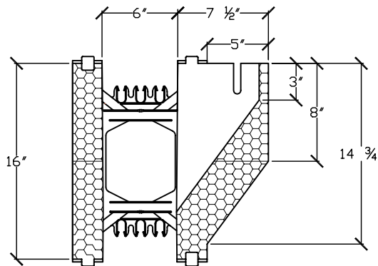
CROSS SECTION OF 6" TO 6" BRICK LEDGE FORM
