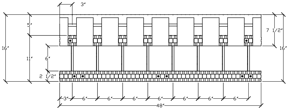
PLAN OF 6" TO 6" BRICK LEDGE FORM
