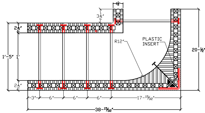
REVERSIBLE 90° CORNER BLOCK LEFT ORIENTED
