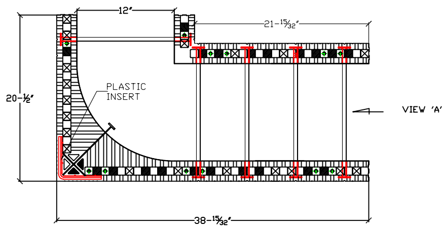
REVERSIBLE 90° CORNER BLOCK RIGHT ORIENTED
