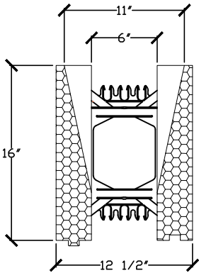
CROSS SECTION OF 6" TAPERED TOP FORM
