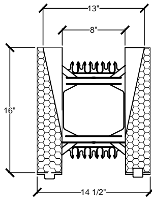
CROSS SECTION OF 8" TAPERED TOP FORM
