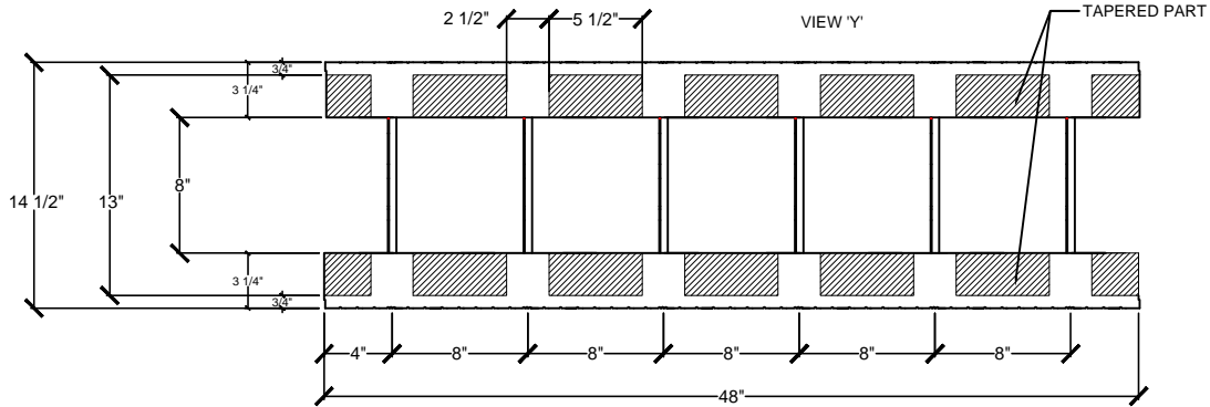
PLAN OF 8" TAPERED TOP FORM
