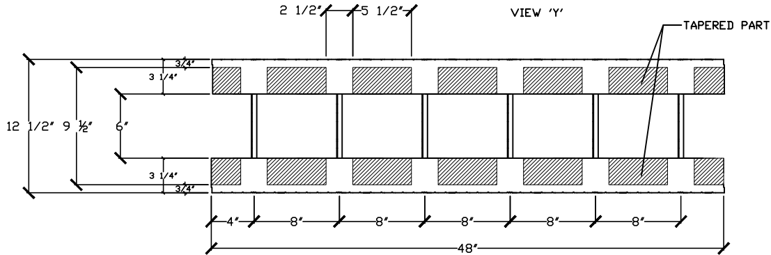
PLAN OF 6" TAPERED TOP FORM
