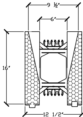
CROSS SECTION OF 6" TAPERED TOP FORM
