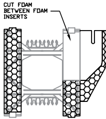
SECTION DETAIL
