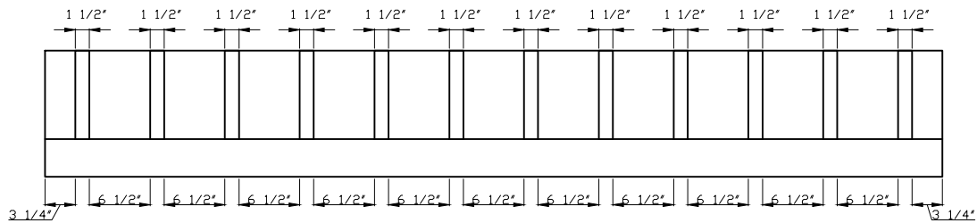
BACK ELEVATION
