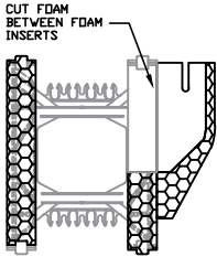
SECTION DETAIL
