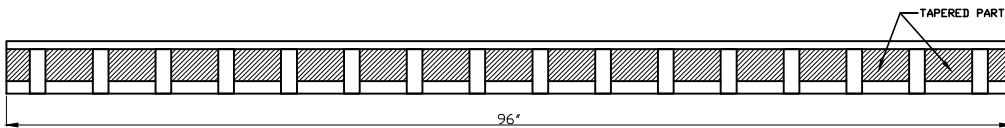
PLAN VIEW
