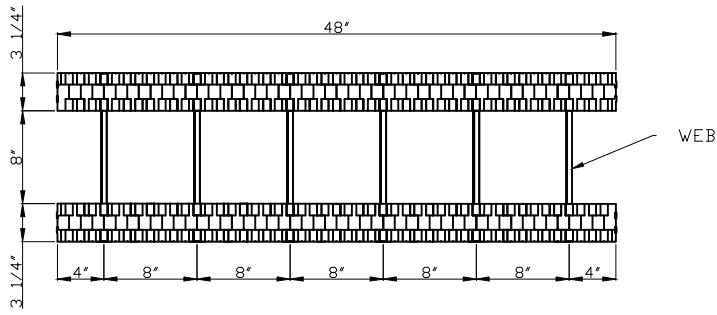
PLAN OF STRAIGHT BLOCK
