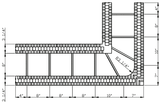
REVERSIBLE 90° CORNER BLOCK LEFT ORIENTED
