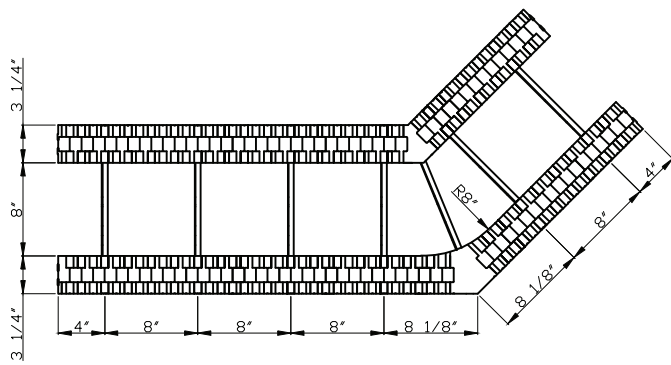
REVERSIBLE 45° CORNER BLOCK LEFT ORIENTED
