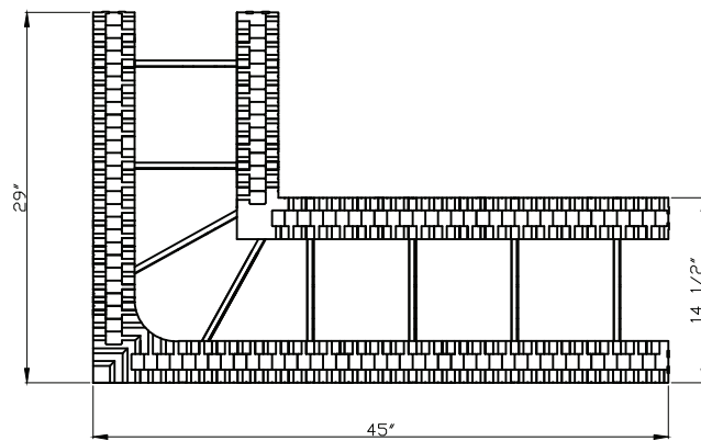
REVERSIBLE 90° CORNER BLOCK RIGHT ORIENTED
