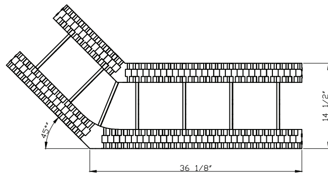
REVERSIBLE 45° CORNER BLOCK RIGHT ORIENTED
