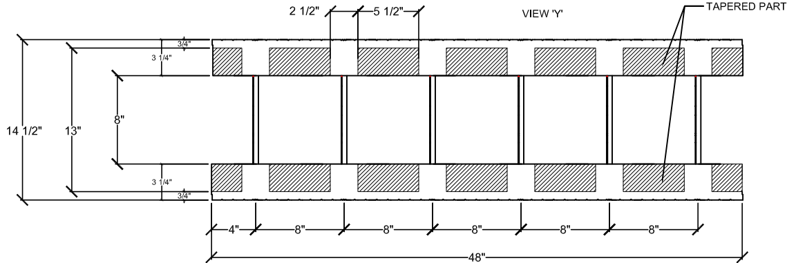
PLAN OF 8" TAPERED TOP FORM
