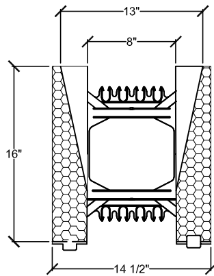
CROSS SECTION OF 8" TAPERED TOP FORM
