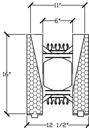
CROSS SECTION OF 6" TAPERED TOP FORM
