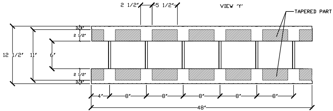
PLAN OF 6" TAPERED TOP FORM
