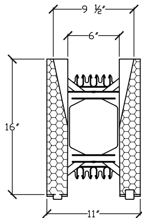
CROSS SECTION OF 6" TAPERED TOP FORM
