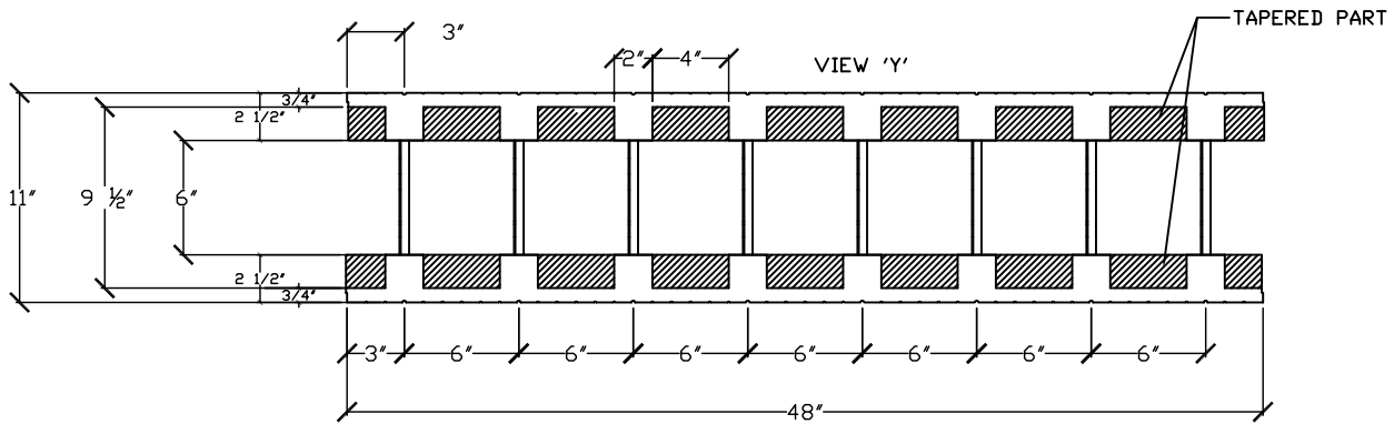
PLAN OF 6" TAPERED TOP FORM
