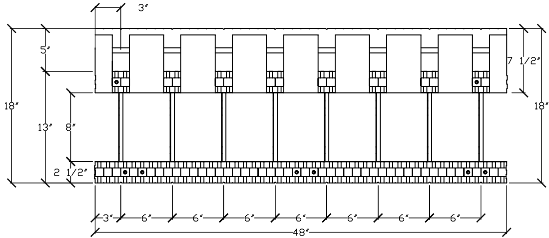
PLAN OF 8" TO 8" BRICK LEDGE FORM
