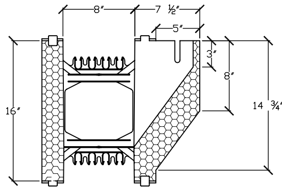
CROSS SECTION OF 8" TO 8" BRICK LEDGE FORM
