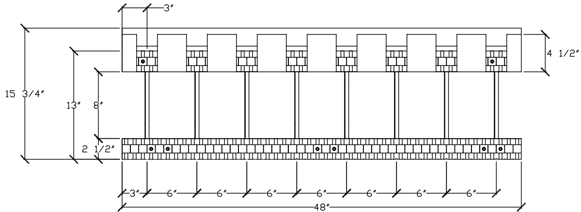
PLAN OF 8" BRICK LEDGE FORM
