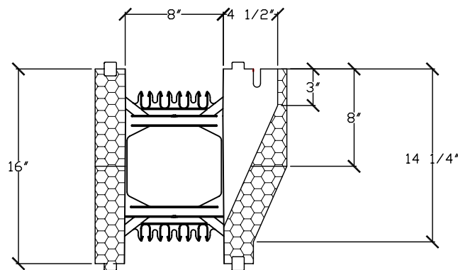
CROSS SECTION OF 8" BRICK LEDGE FORM
