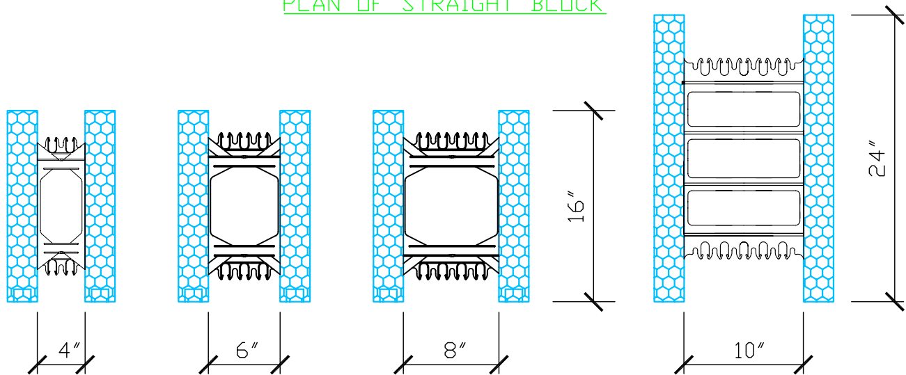
PLAN OF STRAIGHT BLOCK
