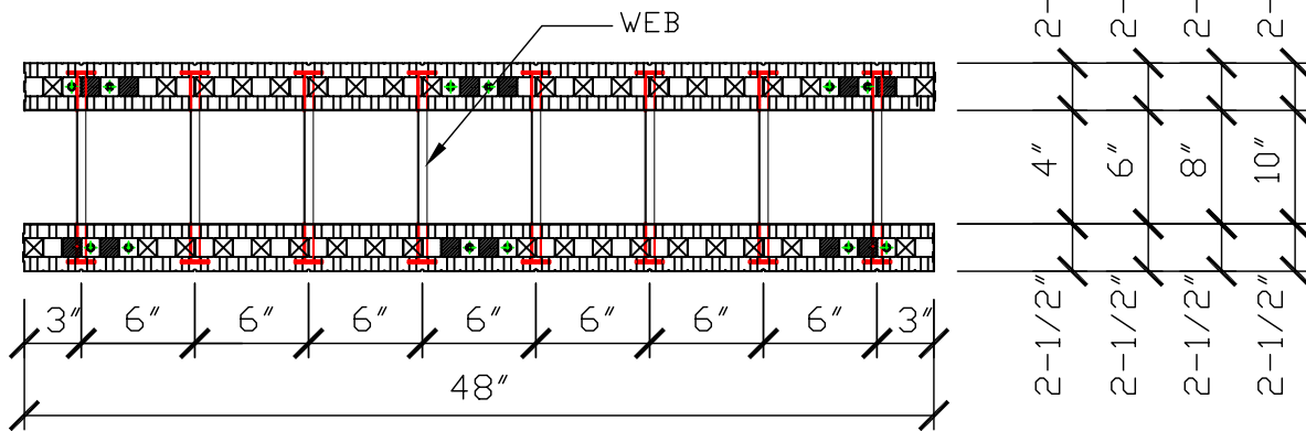
PLAN OF STRAIGHT BLOCK
