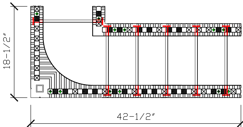
REVERSIBLE 90° CORNER BLOCK RIGHT ORIENTED
