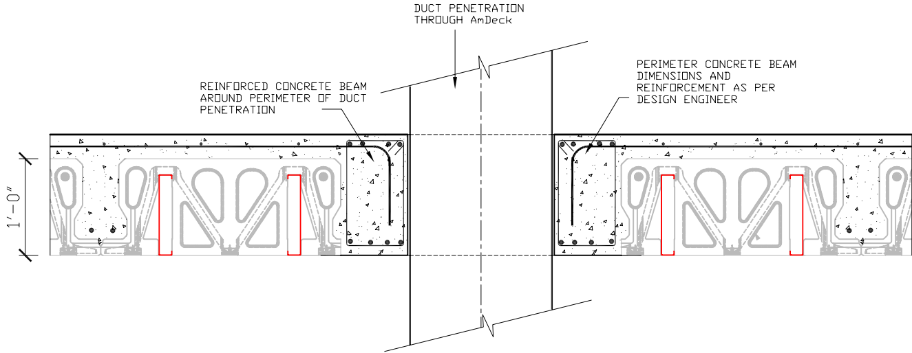
TRANSVERSE SECTION
