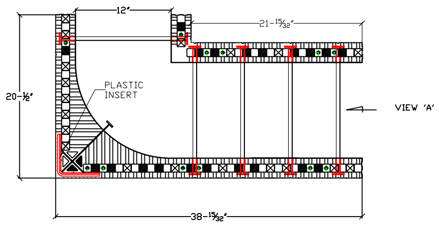
REVERSIBLE 90° CORNER BLOCK RIGHT ORIENTED
